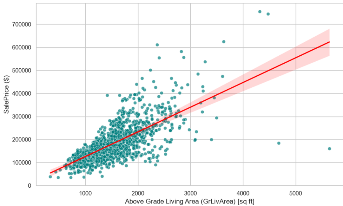
Bivariate Scatter Plot: GrLivArea vs SalePrice
