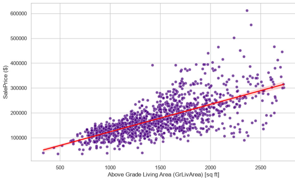
GrLivArea vs SalePrice (After Outlier Removal)
