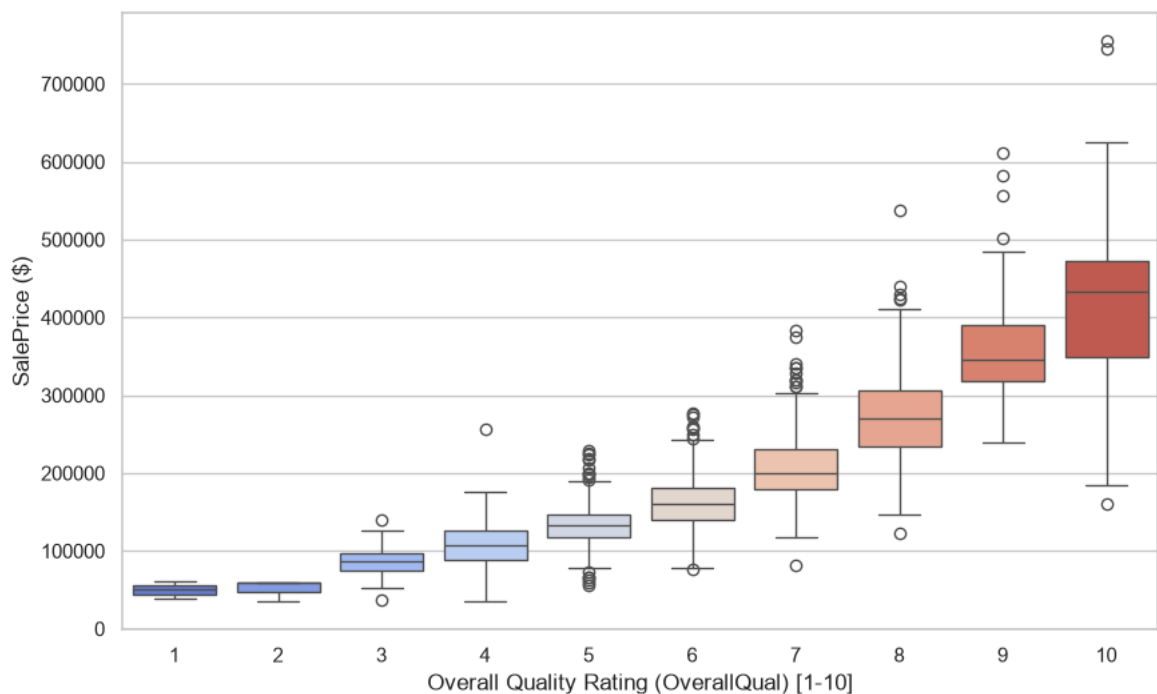
Bivariate Box Plot: SalePrice across OverallQual Rating
